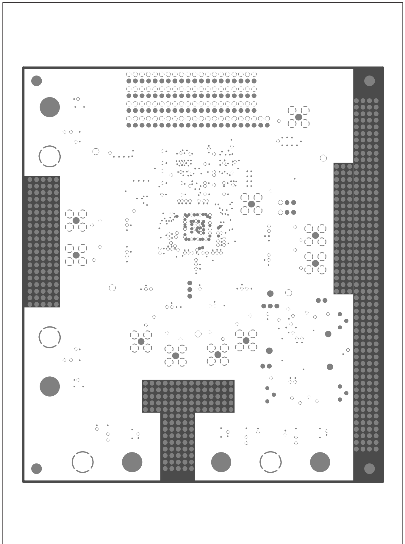
FIGURE 12. EVM Layer 7: Ground Plane II.
